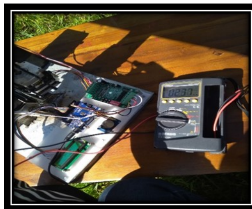
Gambar 4.14 Pengukuran Arus Panel Surya
