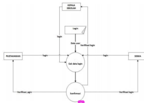
Gambar 3. Diagram level 2 proses login
