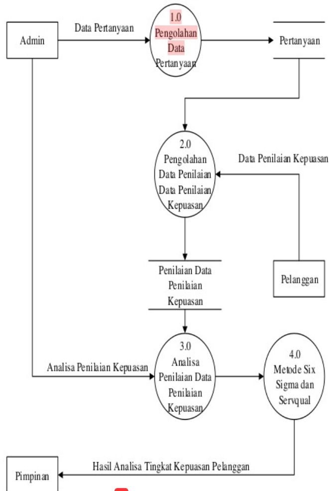
1 Gambar 2. DAD Level 0
