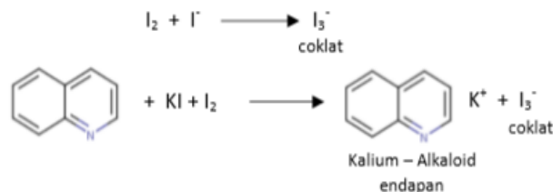
Gambar 3 Reaksi Wagner
