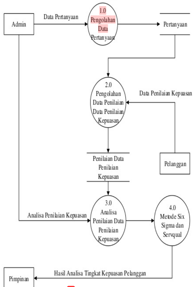
Gambar 2. DAD Level 0
