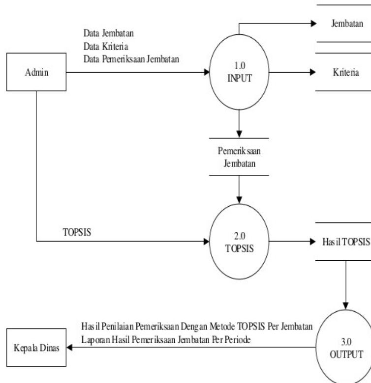
Gambar 3. DFD Level 0
